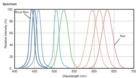
Edison LED Chip Spectrum
