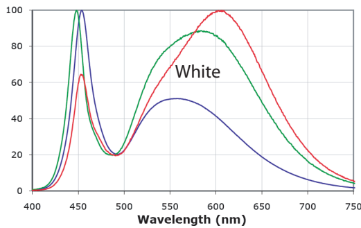
Cree LED Chip Spectrum
